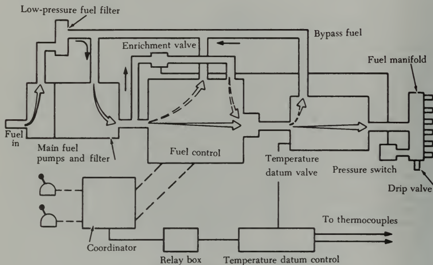
FIGURE 3-43. Allison 501-D13 engine fuel system schematic.
